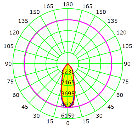
Unit: cd Average Diffuse Angle(50%): 34.0°
